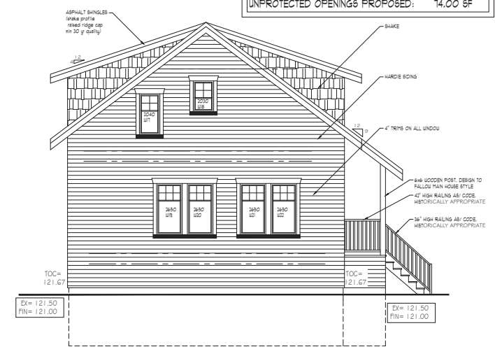
LEFT (WEST) ELEVATION
