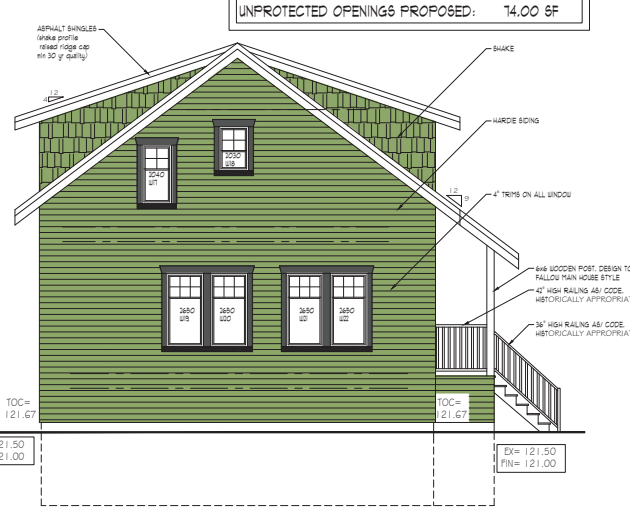
LEFT (WEST) ELEVATION
