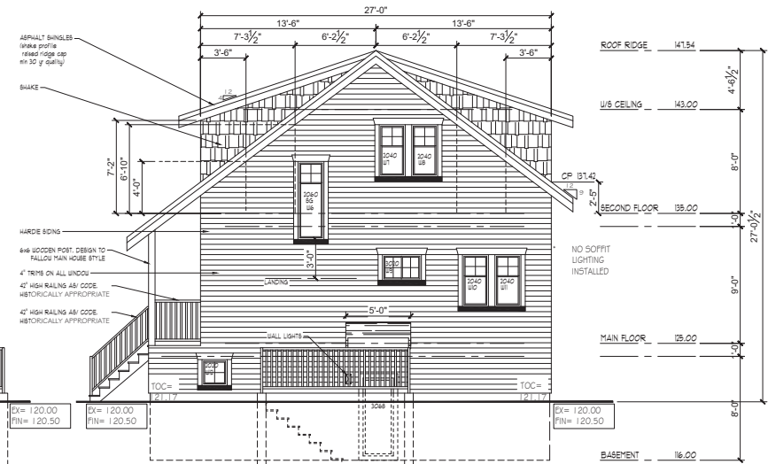
RIGHT (EAST) ELEVATION
